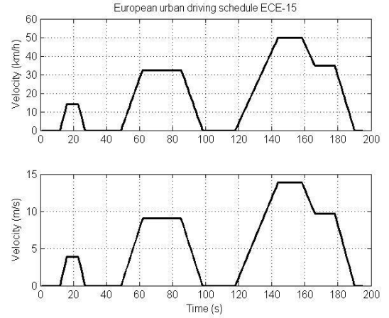
Fig. 2: Driving cycle of European urban driving schedule
